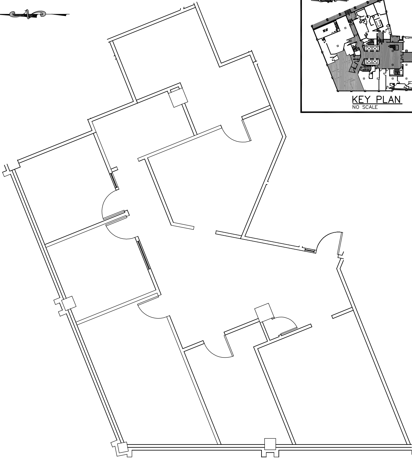
PARTIAL FIRST FLOOR PLAN SCALE: 1/8" = 1'-0"
