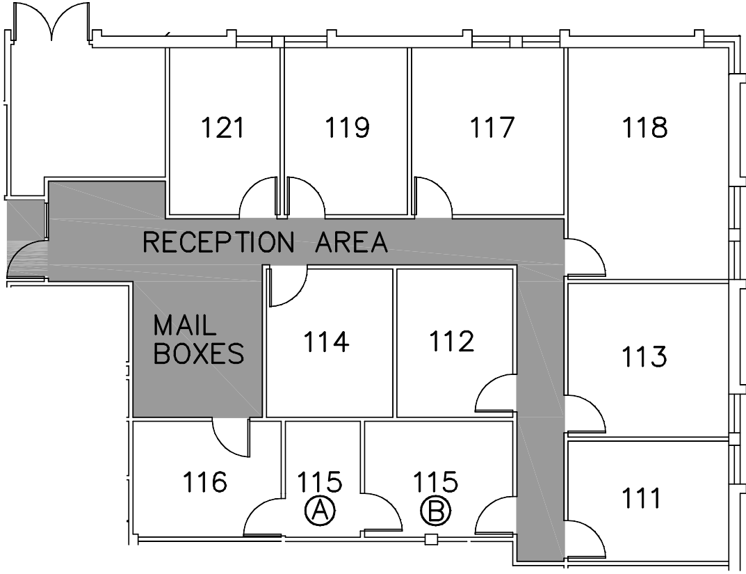
PARTIAL FIRST FLOOR PLAN SCALE: \frac{3}{32}'' = 1'-0''
