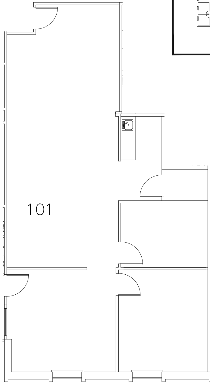
PARTIAL FIRST FLOOR PLAN SCALE: 1/8"=1'-0"
