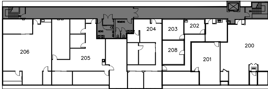
SECOND FLOOR PLAN SCALE: 1/32" = 1'-0"
