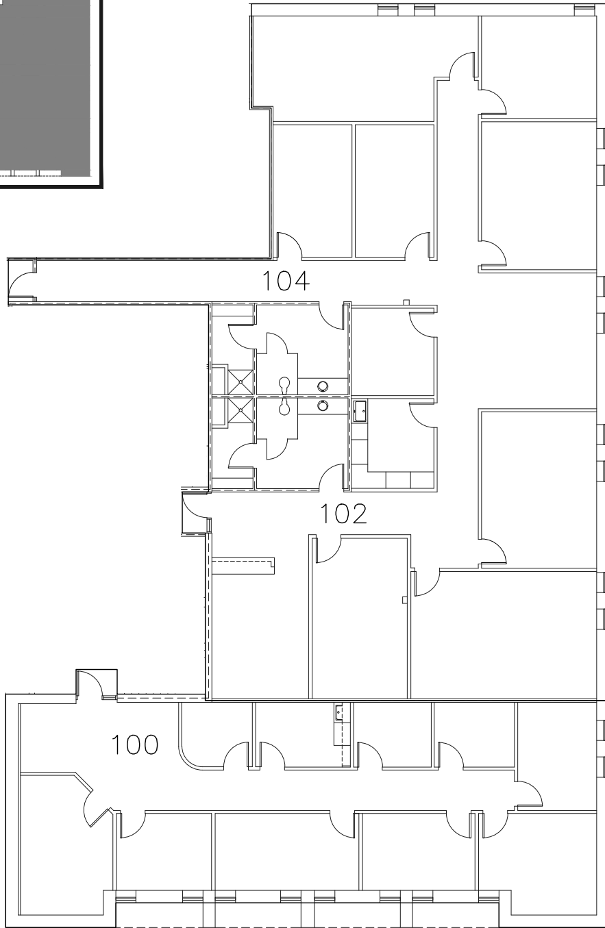
PARTIAL FIRST FLOOR PLAN SCALE: 1/16"=1'-0"
