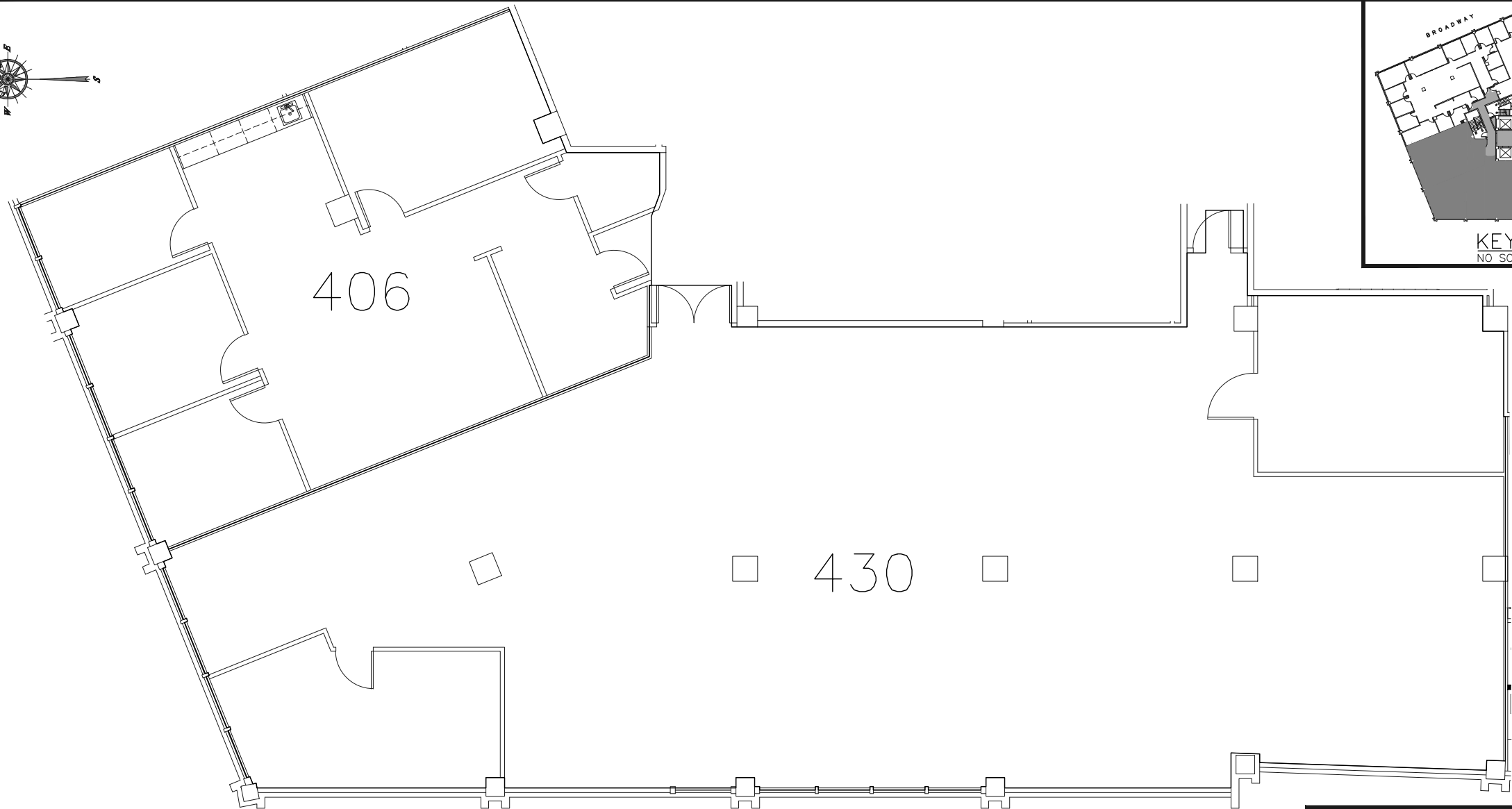
FOURTH FLOOR PLAN SCALE: 3/32" = 1'-0"
