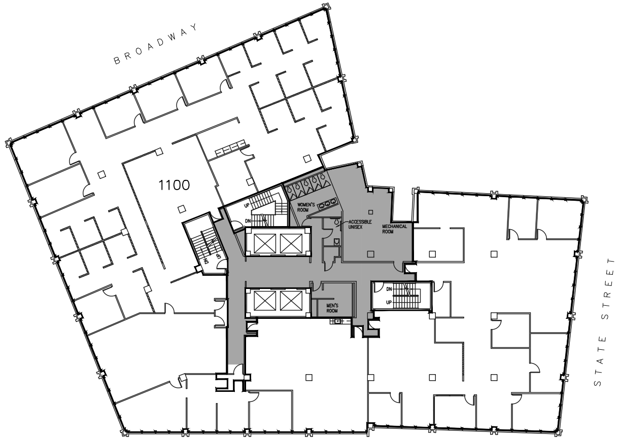
ELEVENTH FLOOR PLAN SCALE: 1/32" = 1'-0"
