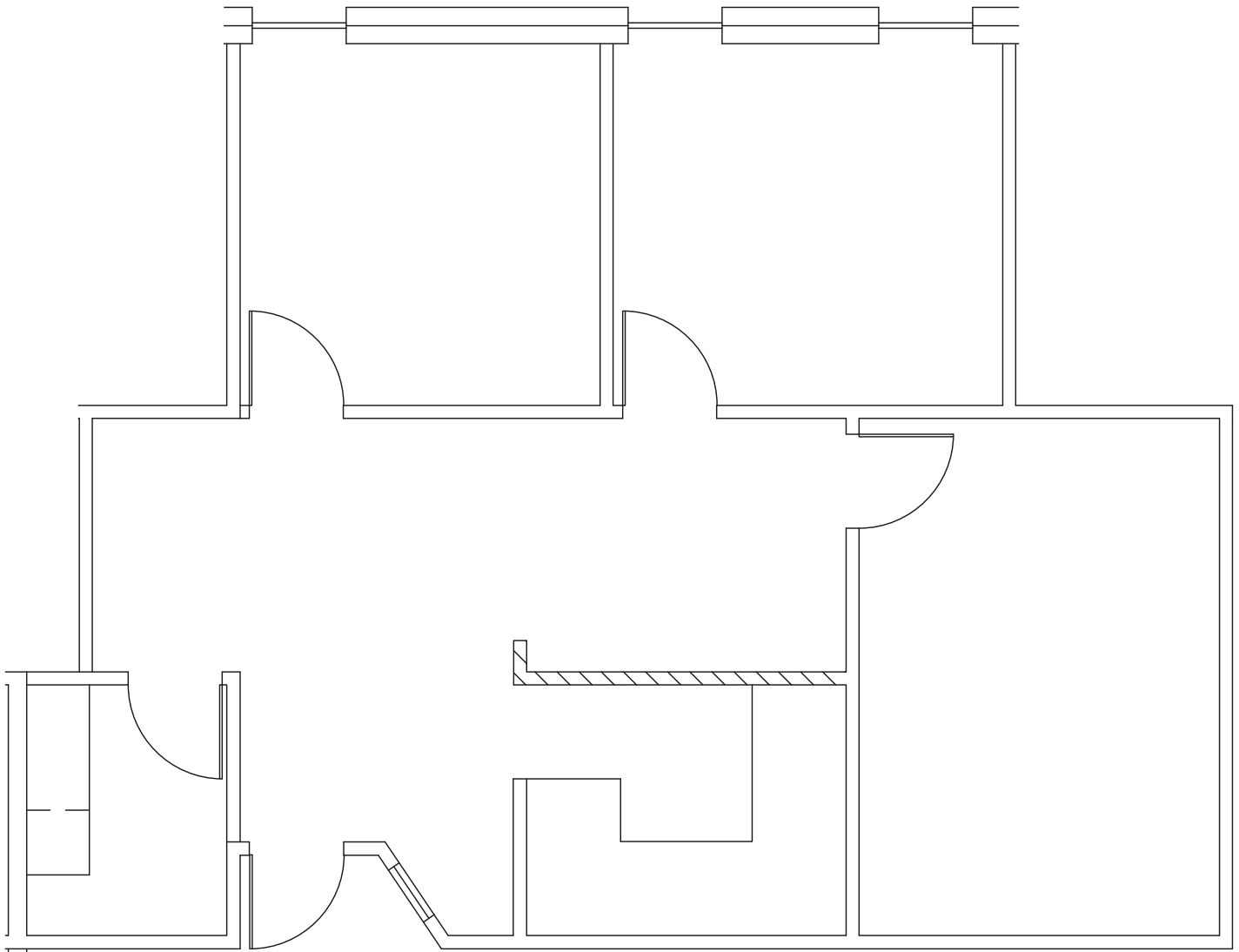
PARTIAL SECOND FLOOR PLAN SCALE: 3/16"=1'-0"
